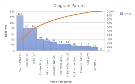
Gambar 3. Diagram Pareto
