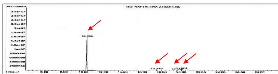
Figure 8. GC-MS Chromatogram Interactions between BC microsymbionts with Naphthalene Contact period of 25 days
